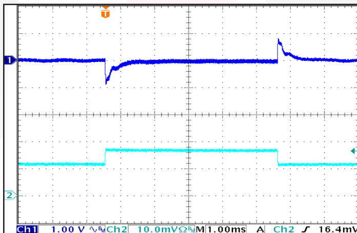
Figure 11: Output Voltage Response to Step-Change in Load Current , (50%-75%-50% of I_{out(max)} ; dI/dt = 0.5 A/µs). Load cap: 1 µF ceramic and 100 µF electrolytic capacitors. Ch 1: \Delta V_{out} (1 V/div); Ch 2: I_{out} (10 A/div). Timescale: 1.00ms/div.
