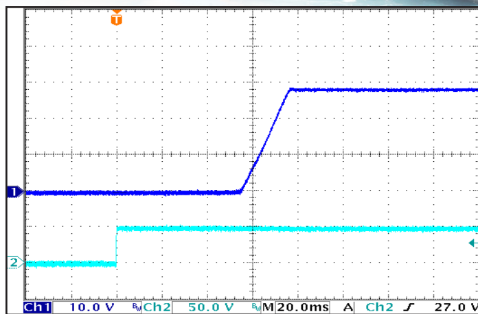
Figure 8: Turn-On Transient , at full resistive load and zero output capacitance initiated by V_{in} . Ch 1: V_{out} (10 V/div); Ch 2: V_{in} (50 V/div). Timescale: 20.0ms/div.
