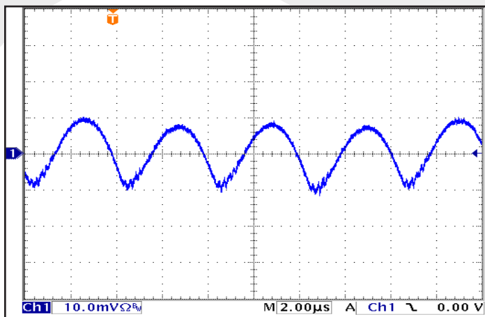
Figure 9: Input Terminal Current Ripple , i_C , at full rated output current and nominal input voltage with SynQor MCOTS filter module (500 mA/div). Bandwidth: 20 MHz. Timescale: 2.00µs/div. See Figure 13.
