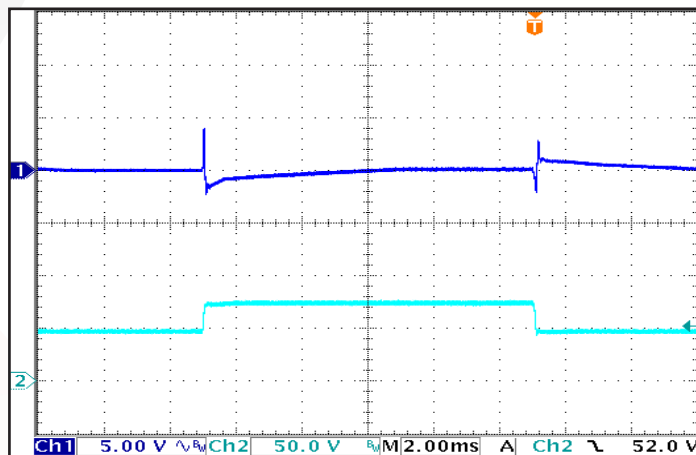
Figure 12: Output Voltage Response to Step-Change in Input Voltage , (500 V/ms). Load cap: 100 µF electrolytic output capacitance. Ch 1: V_{out} (5 V/div), Ch 2: V_{in} (50 V/div). Timescale: 2.00ms/div.
