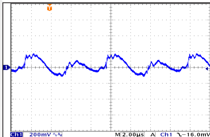
Figure 10: Output Voltage Ripple , V_{out} , at nominal input voltage and rated load current (200 mV/div). Load capacitance: 1 µF ceramic and 100 µF electrolytic capacitors. Bandwidth: 20 MHz. Timescale: 2.00µsec/div. See Figure 13.
